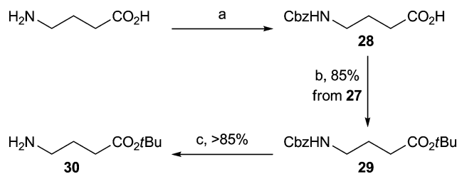
Scheme 7 Reagents and conditions: a) BnOCOC 1 , NaOH/H 2 O, r.t.; b) t BuOH, DCC, DMAP, CH 2 Cl 2 , r.t.; c) H 2 , Pd/C, MeOH, r.t.
